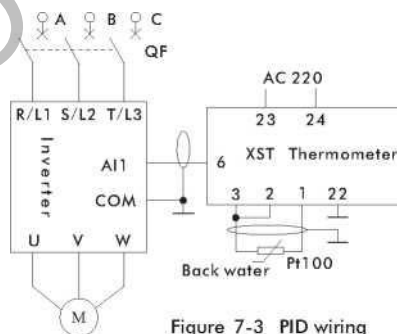
Figure 7-3 PID wiring
