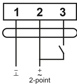
AC/DC 21...27V
